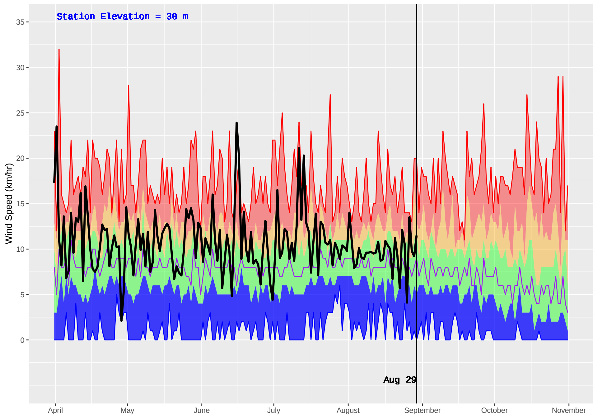
CEDAR (59) : Historical (1989–2016) and Current (2018) Daily Wind Speed
